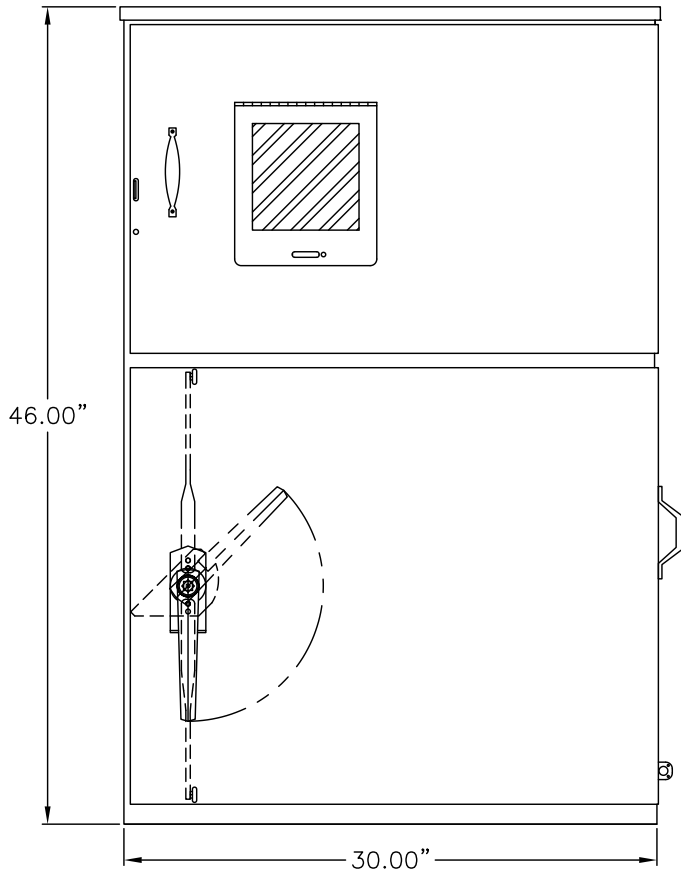
PANEL ELEVATION
