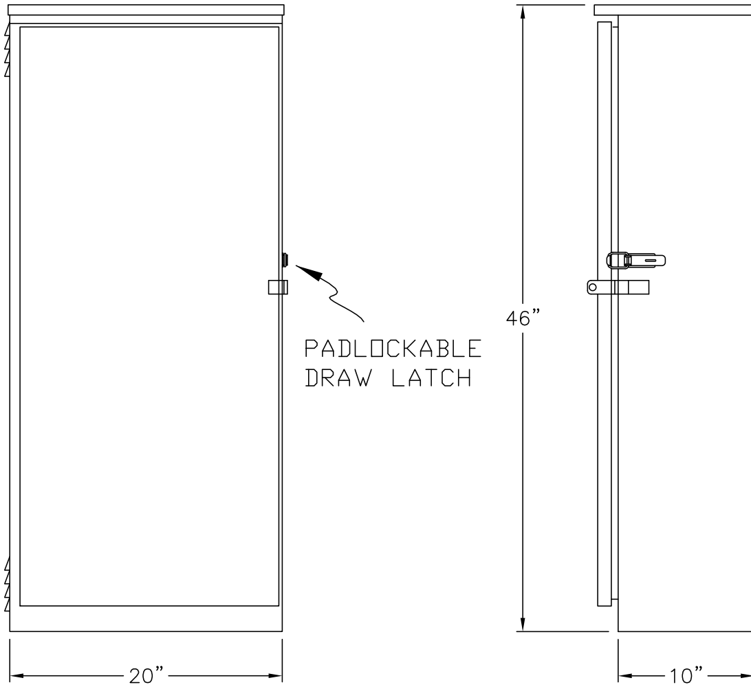
FRONT VIEW
