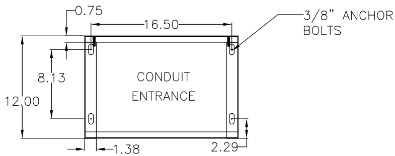
BASE PLAN
