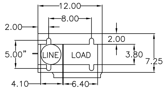
BASE PLAN
