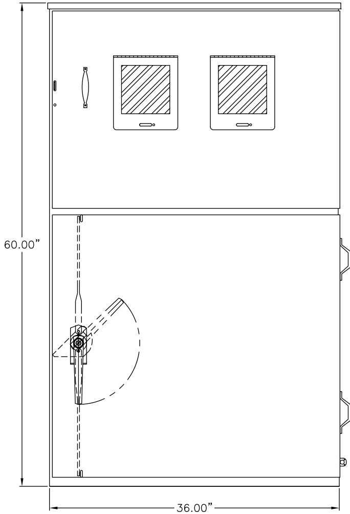
PANEL ELEVATION
